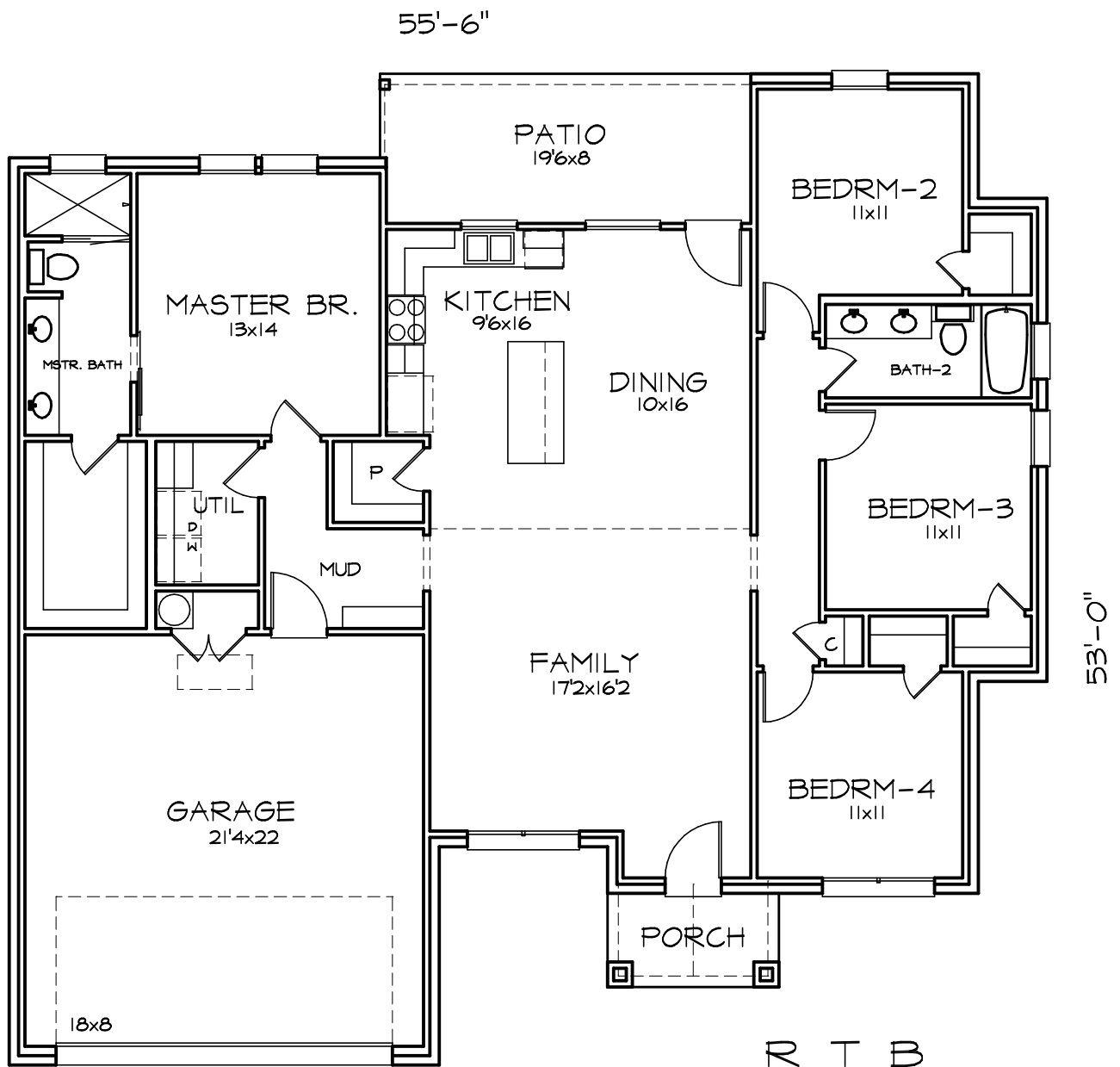
FLOOR PLAN 1776 SF
