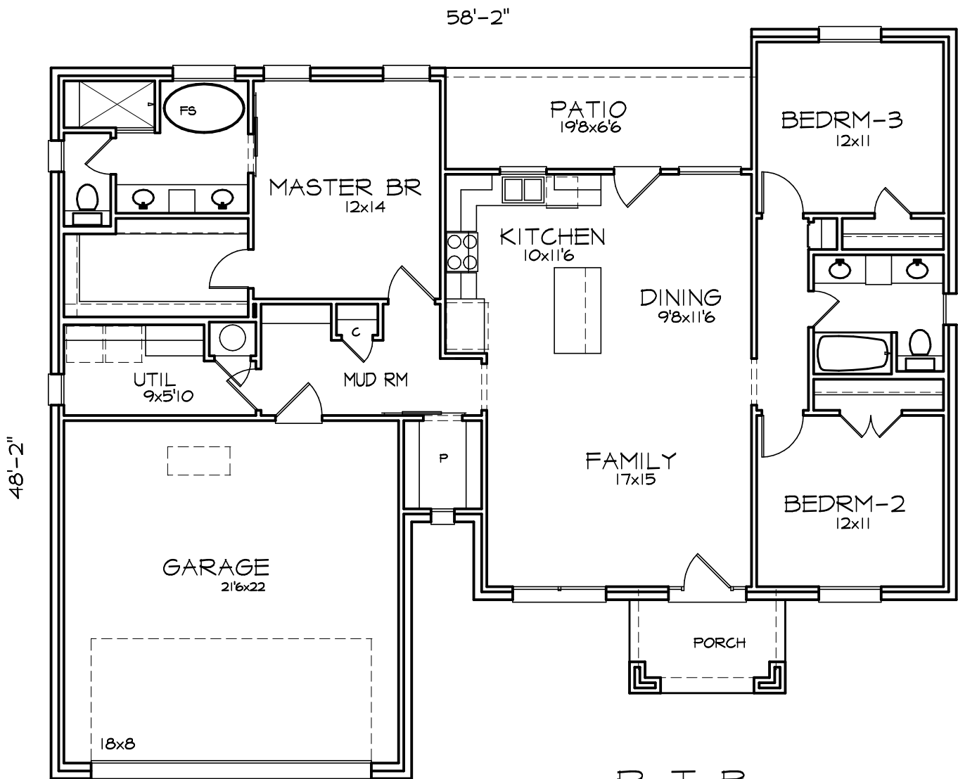
FLOOR PLAN 101231611-L 1611 SF
